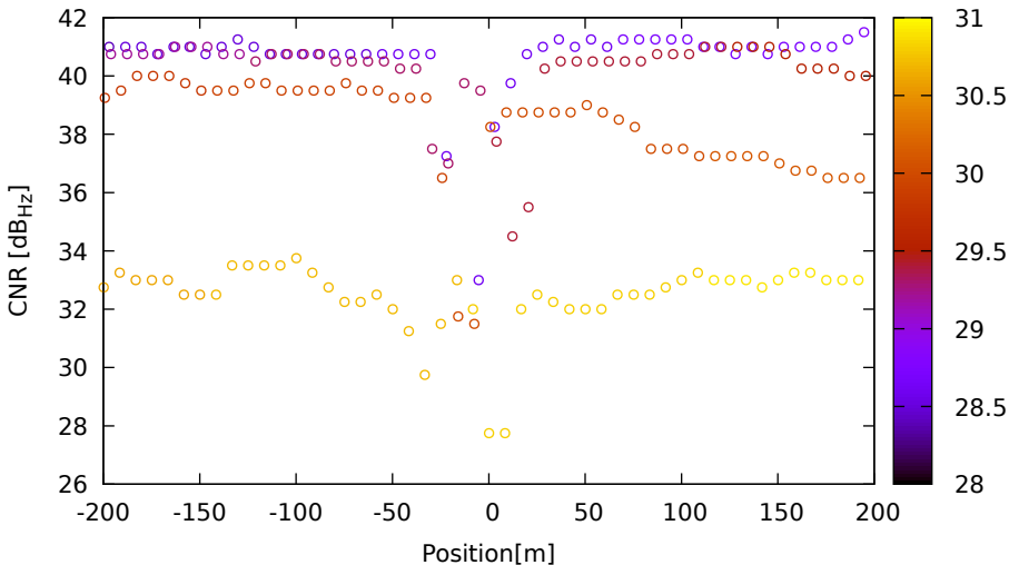
CNR vs position for R03 (G1) on XiaomiMi8 - DOY 263 jam. 2
