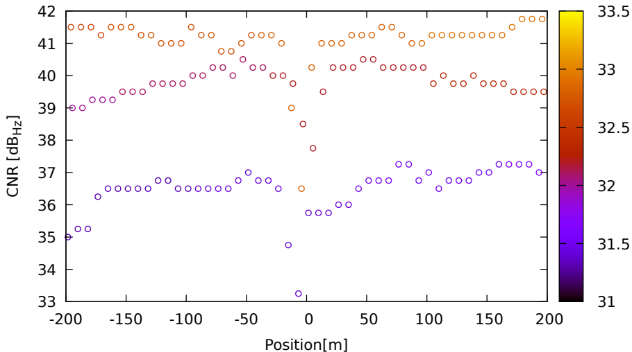
CNR vs position for R03 (G1) on XiaomiMi8 - DOY 263 jam. 3
