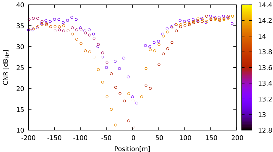
CNR vs position for R11 (G1) on XiaomiMi8 - DOY 263 jam. 1
