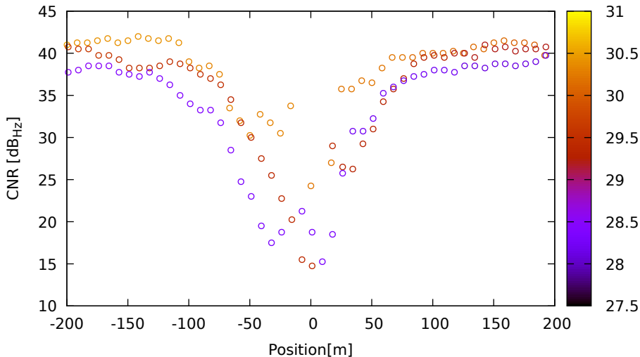
CNR vs position for R24 (G1) on XiaomiMi8 - DOY 263 jam. 1
