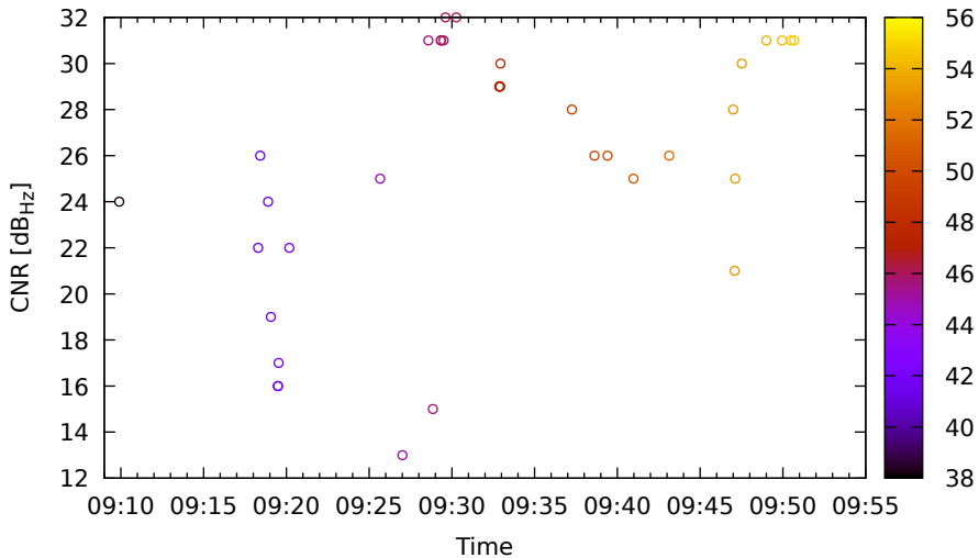
Timeline for E05 (E5a) on HuaweiP40 - DOY 262
