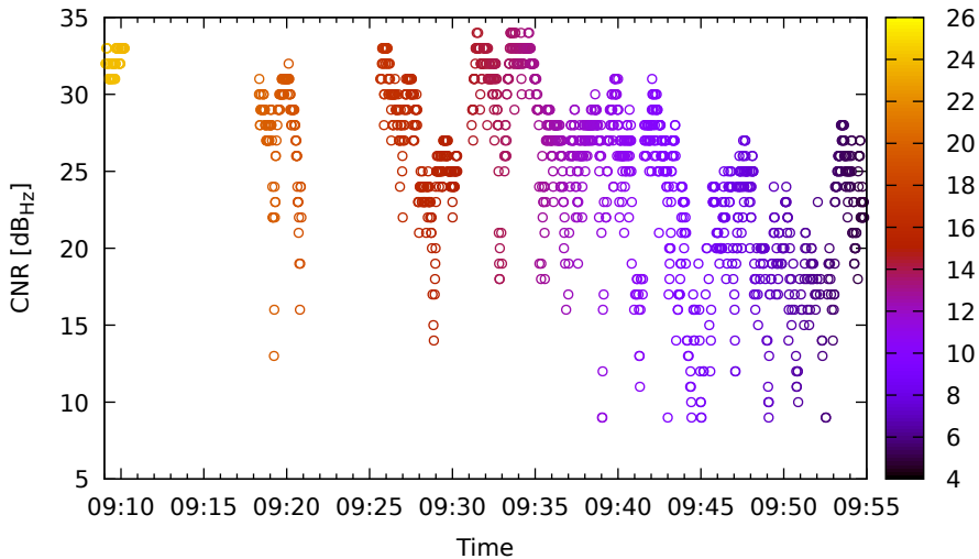
Timeline for G08 (L1) on HuaweiP40 - DOY 262
