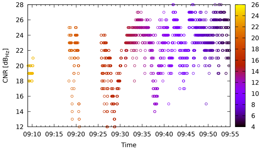
Timeline for G08 (L5) on HuaweiP40 - DOY 262
