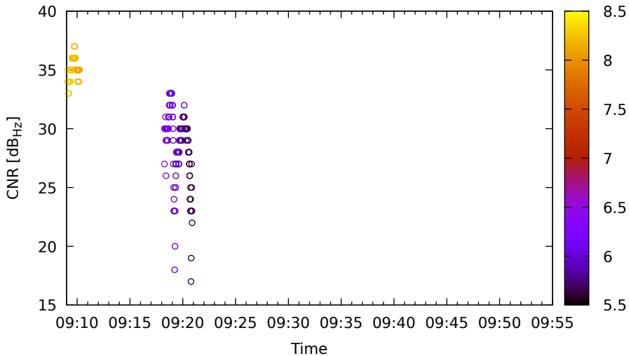
Timeline for G14 (L1) on HuaweiP40 - DOY 262
