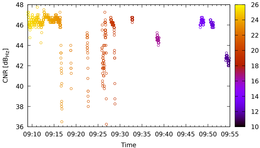
Timeline for E04 (E5b) on LeicaGS15 - DOY 262
