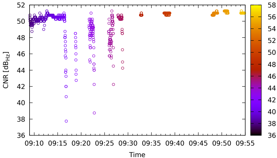
Timeline for E05 (E5b) on LeicaGS15 - DOY 262
