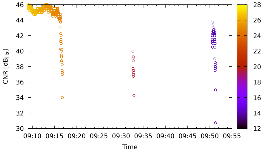
Timeline for E11 (E1) on LeicaGS15 - DOY 262
