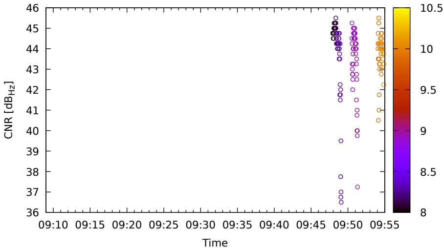
Timeline for E15 (E1) on LeicaGS15 - DOY 262
