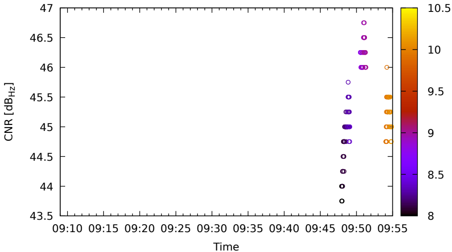
Timeline for E15 (E5b) on LeicaGS15 - DOY 262
