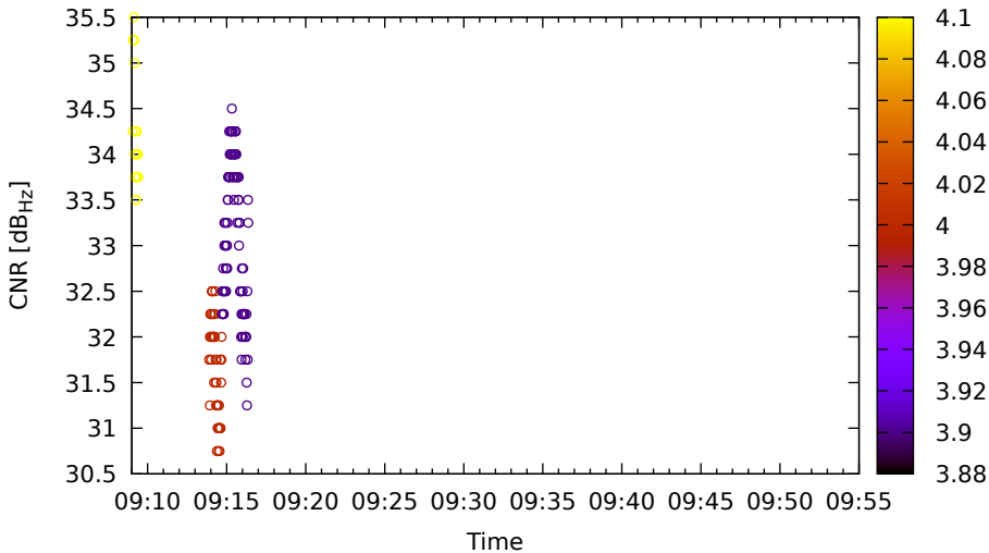
Timeline for E27 (E5) on LeicaGS15 - DOY 262
