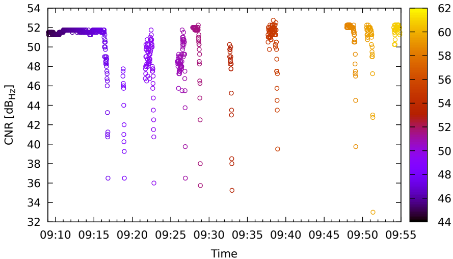
Timeline for E34 (E1) on LeicaGS15 - DOY 262
