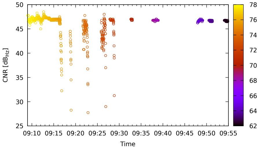
Timeline for E36 (E5) on LeicaGS15 - DOY 262
