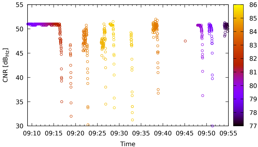
Timeline for G01 (L1) on LeicaGS15 - DOY 262
