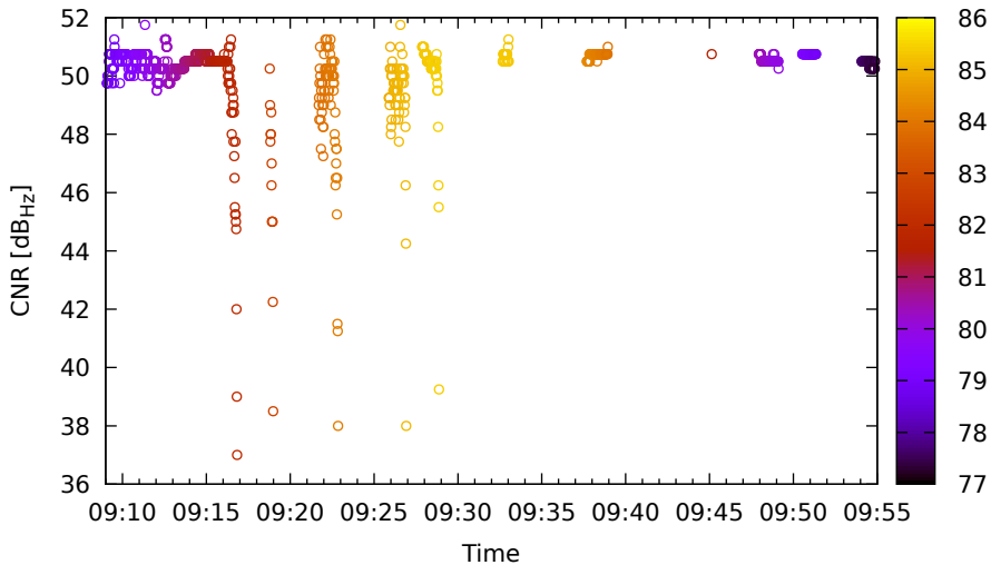
Timeline for G01 (L5) on LeicaGS15 - DOY 262
