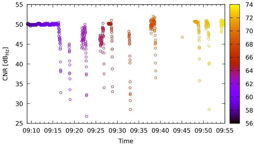
Timeline for G03 (L2) on LeicaGS15 - DOY 262
