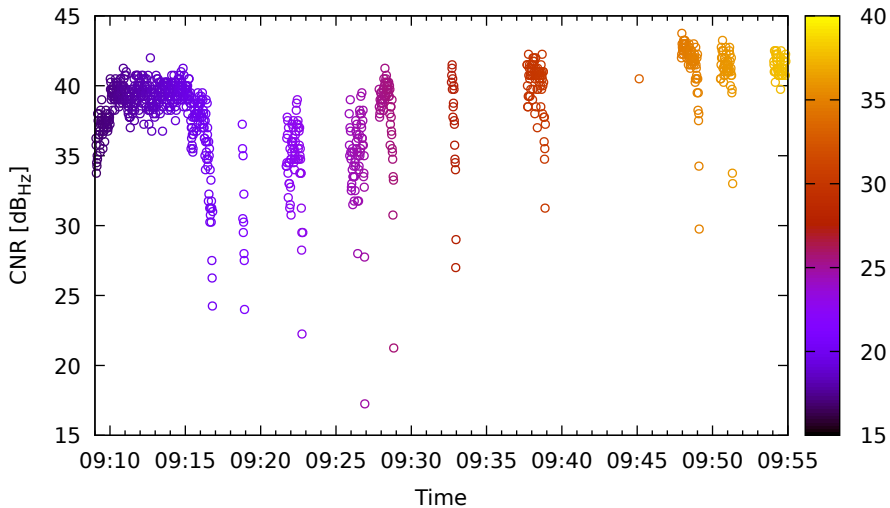
Timeline for G04 (L2) on LeicaGS15 - DOY 262
