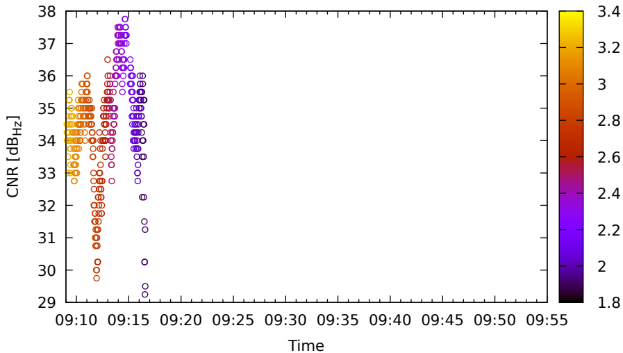
Timeline for R15 (G1) on LeicaGS15 - DOY 262
