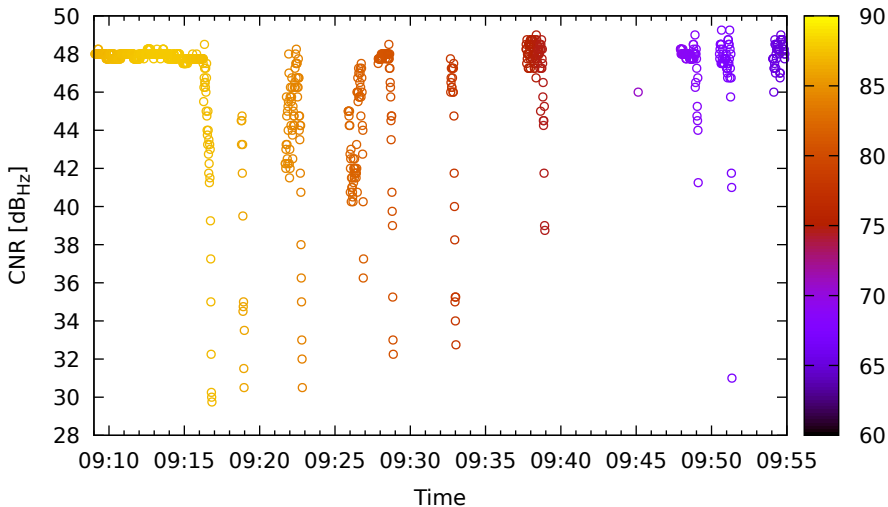
Timeline for R23 (G1) on LeicaGS15 - DOY 262
