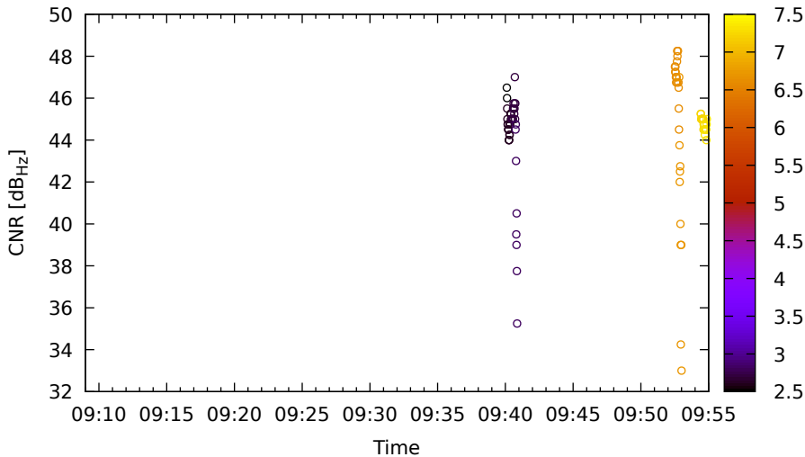
Timeline for E03 (E1) on LeicaGS15 - DOY 262
