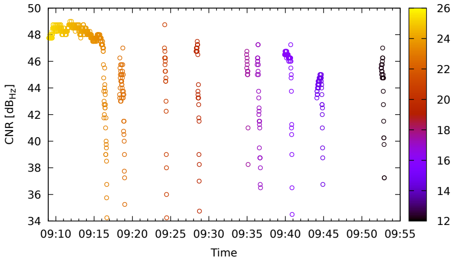
Timeline for E04 (E1) on LeicaGS15 - DOY 262
