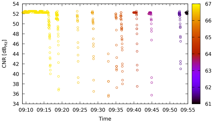
Timeline for E09 (E1) on LeicaGS15 - DOY 262
