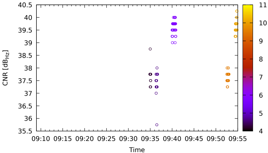
Timeline for E15 (E5a) on LeicaGS15 - DOY 262
