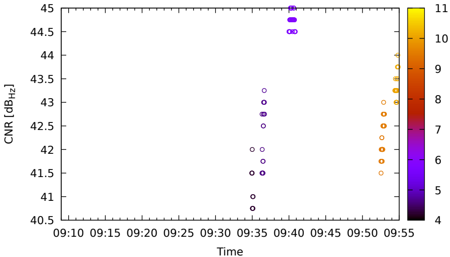
Timeline for E15 (E5b) on LeicaGS15 - DOY 262
