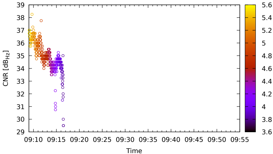
Timeline for E30 (E5) on LeicaGS15 - DOY 262
