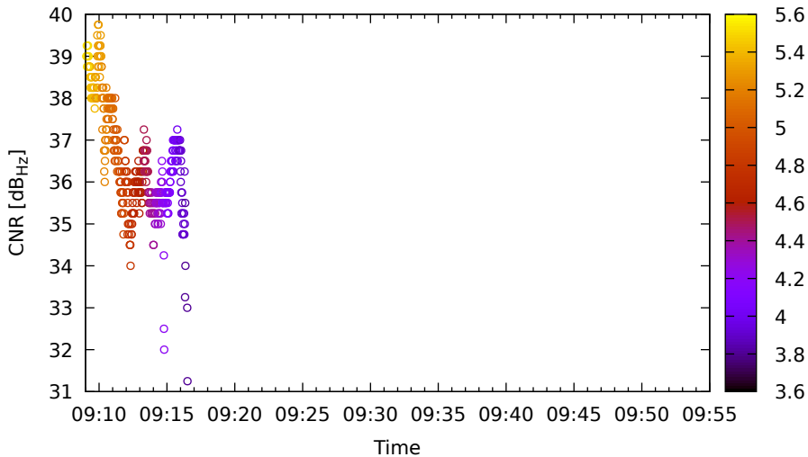
Timeline for E30 (E5a) on LeicaGS15 - DOY 262
