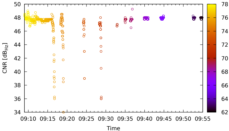
Timeline for E36 (E5a) on LeicaGS15 - DOY 262
