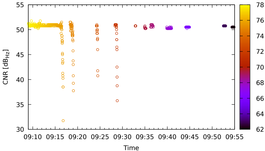
Timeline for E36 (E5b) on LeicaGS15 - DOY 262
