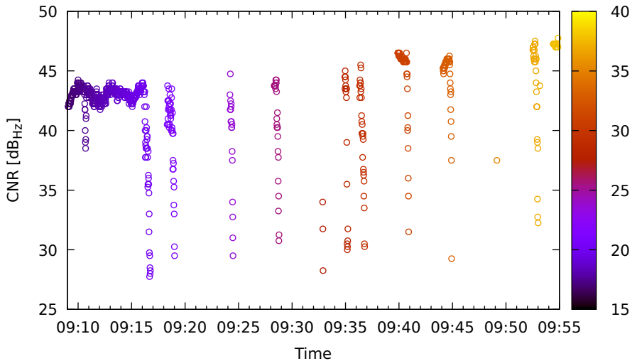
Timeline for G04 (L1) on LeicaGS15 - DOY 262
