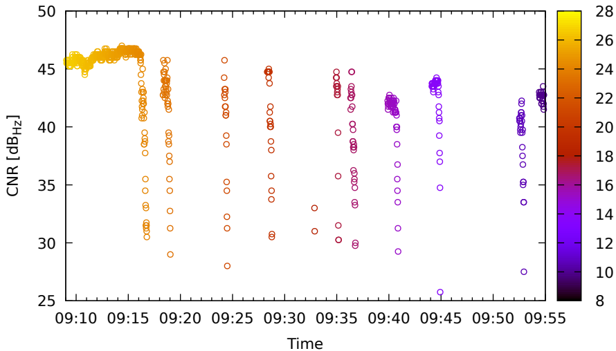
Timeline for G32 (L1) on LeicaGS15 - DOY 262
