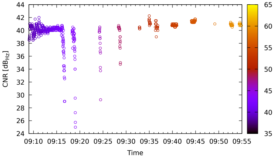
Timeline for R01 (G2) on LeicaGS15 - DOY 262
