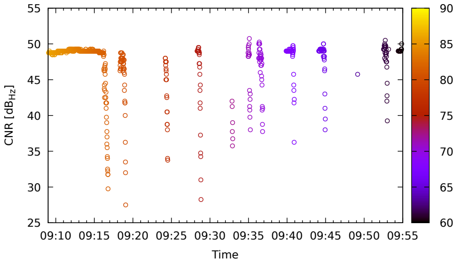
Timeline for R08 (G1) on LeicaGS15 - DOY 262
