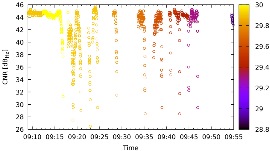
Timeline for C06 (B1) on LeicaGS18 - DOY 262
