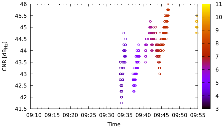
Timeline for E15 (E5) on LeicaGS18 - DOY 262
