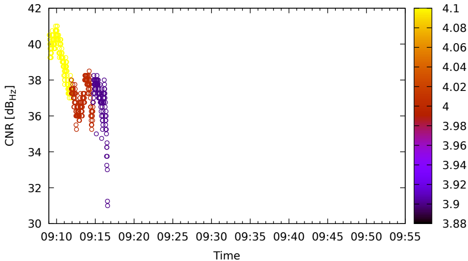
Timeline for E27 (E1) on LeicaGS18 - DOY 262
