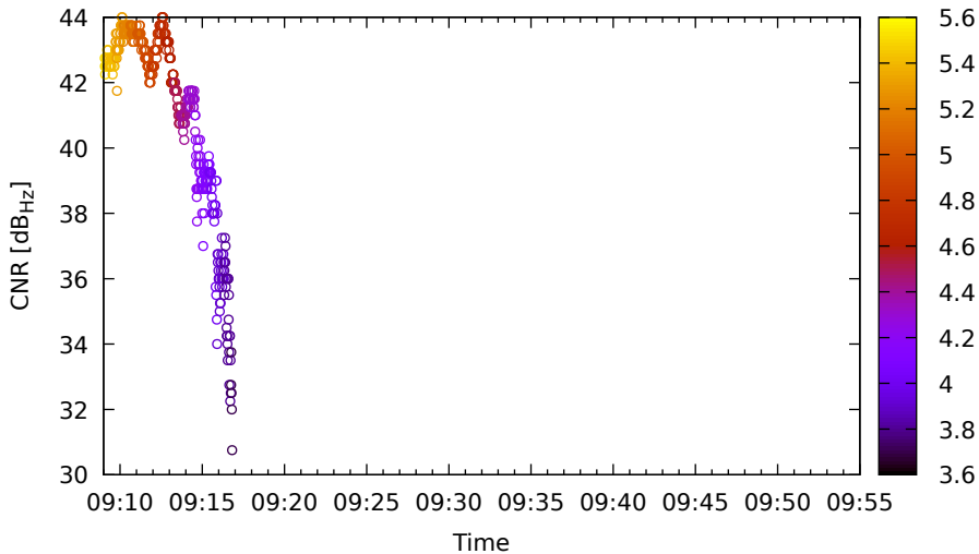
Timeline for E30 (E5a) on LeicaGS18 - DOY 262
