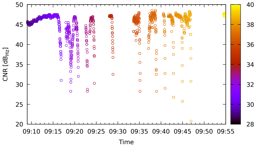
Timeline for G17 (L1) on LeicaGS18 - DOY 262
