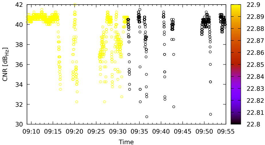
Timeline for C05 (B1) on LeicaGS18 - DOY 262
