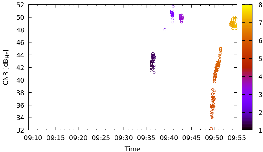
Timeline for E03 (E5b) on LeicaGS18 - DOY 262
