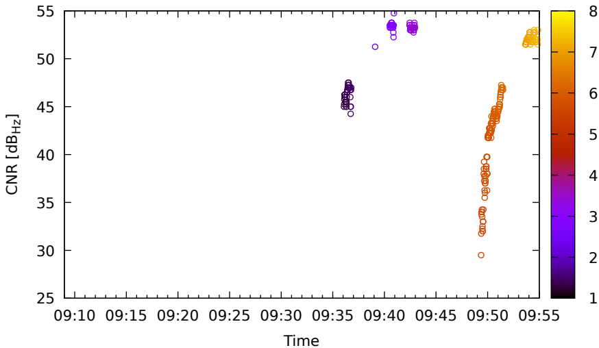
Timeline for E03 (E8) on LeicaGS18 - DOY 262
