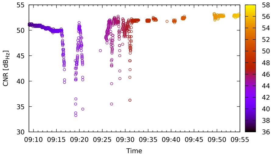
Timeline for E05 (E5a) on LeicaGS18 - DOY 262
