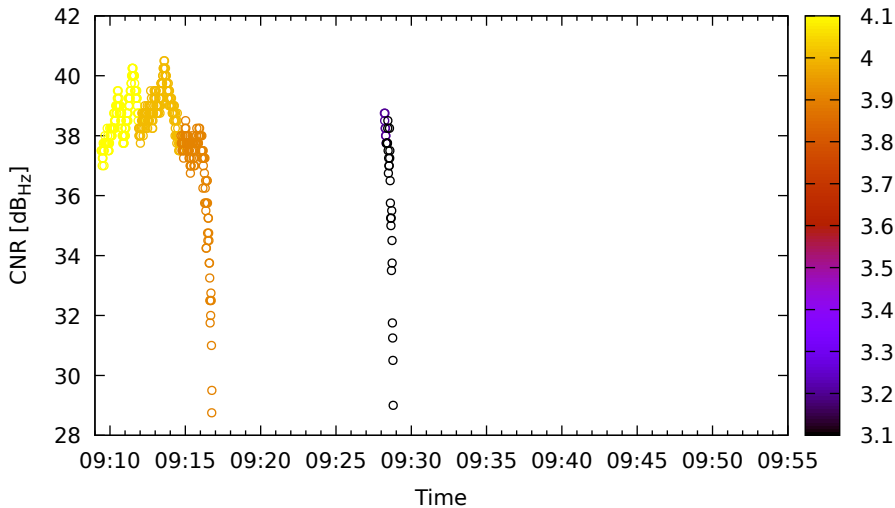
Timeline for E27 (E5a) on LeicaGS18 - DOY 262
