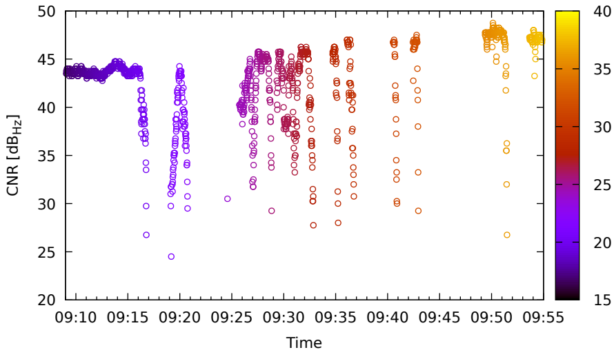
Timeline for G04 (L1) on LeicaGS18 - DOY 262
