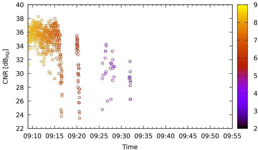
Timeline for G14 (L2) on LeicaGS18 - DOY 262
