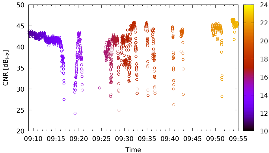
Timeline for G31 (L1) on LeicaGS18 - DOY 262
