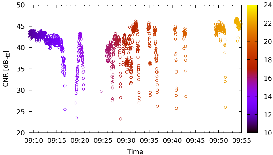
Timeline for G31 (L2) on LeicaGS18 - DOY 262
