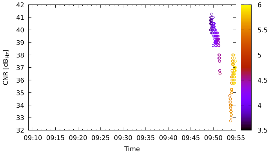
Timeline for R02 (G2) on LeicaGS18 - DOY 262
